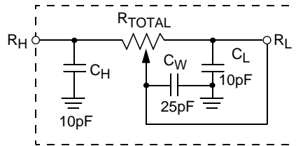
Circuit #2 SPICE Macro Model
