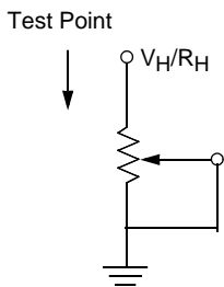
Test Circuit #1
