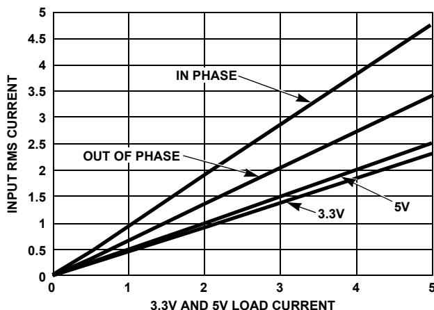
FIGURE 18. INPUT RMS CURRENT vs LOAD
