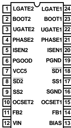
ISL6445 (QSOP) TOP VIEW
