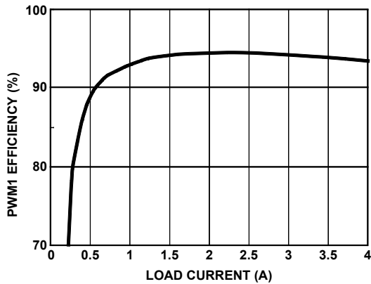
FIGURE 11. PWM1 EFFICIENCY vs LOAD (3.3V), VIN = 5V
