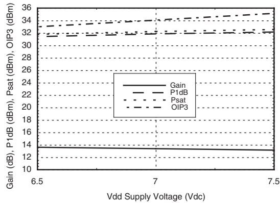
Gain, Power & OIP3 vs. Supply Voltage @ 15 GHz
