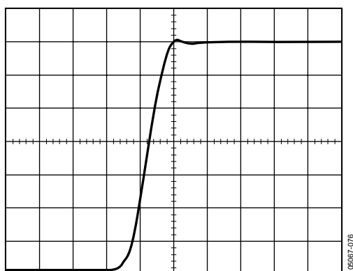
Figure 76. Output Signal after Adaptive Filter Control
