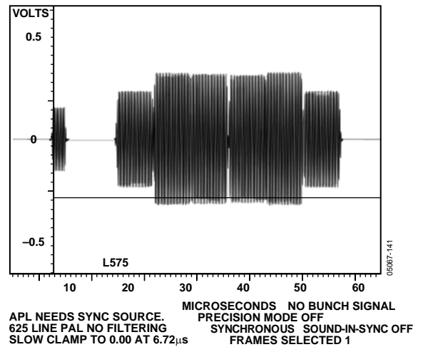
Figure 141. PAL Chroma
