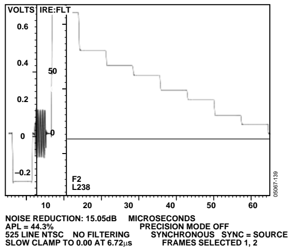
Figure 139. NTSC Luma
