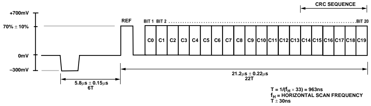
Figure 92. Progressive Scan 525p CGMS Waveform (Line 41)
