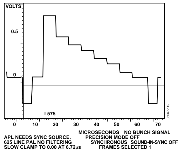
Figure 142. PAL Luma
