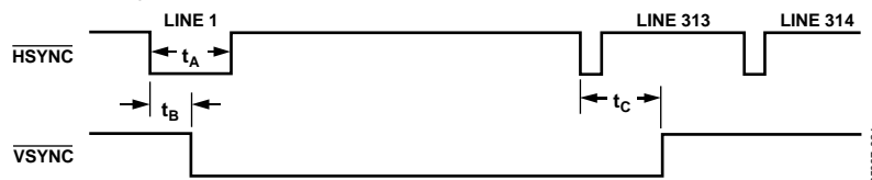
Figure 48. Timing Register 1 in PAL Mode
