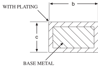
6 PIN SC-70
