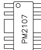
PM-SOP ™ Plastic Package
