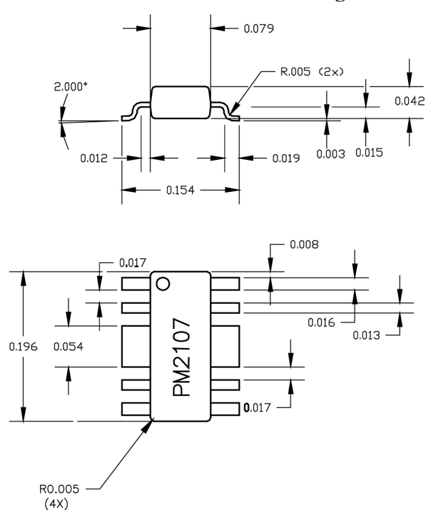
PM-SOP™ Outline Drawing
