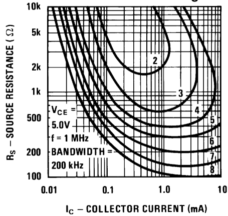
Contours of Constant Narrow Band Noise Figure
