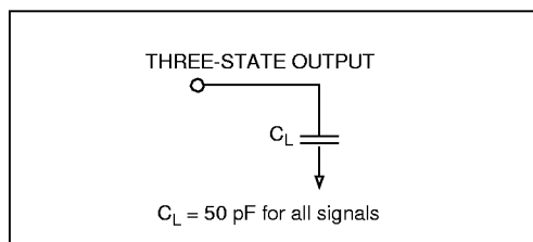
Figure 11. Test Load Circuit for Three-State Output Pins
