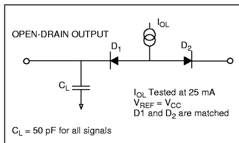
Figure 12. Test Load Circuit for Open-Drain Output Pins
