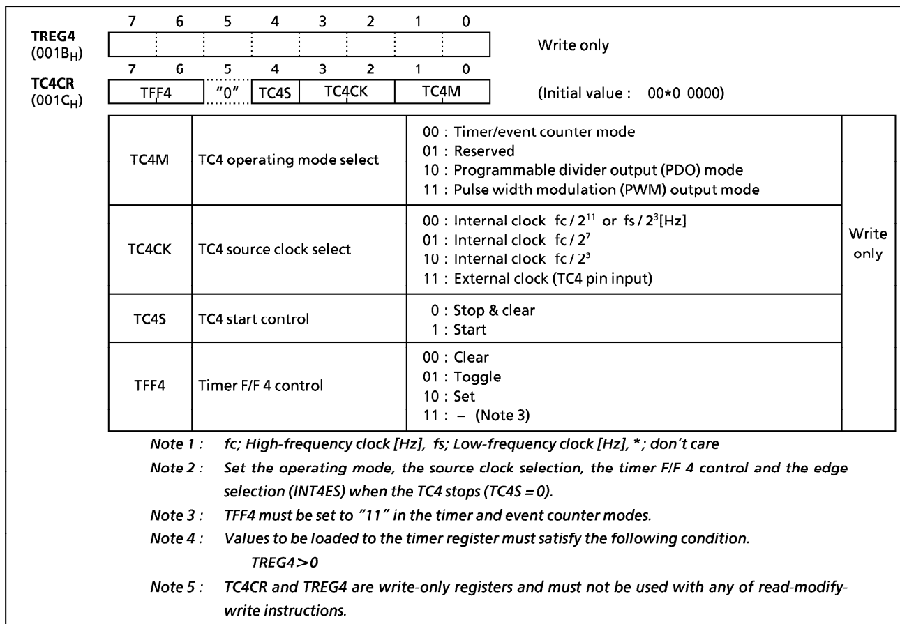
Figure 2-34. Timer Register 4 and TC4 Control Register
