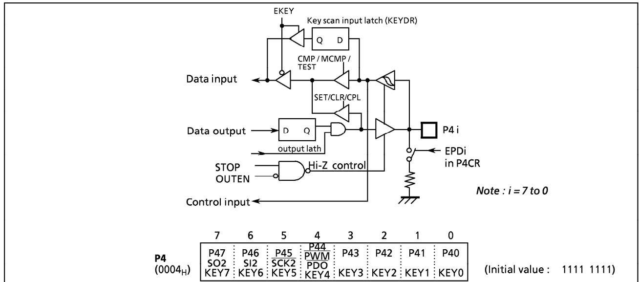
Figure 2-7. Port P4
