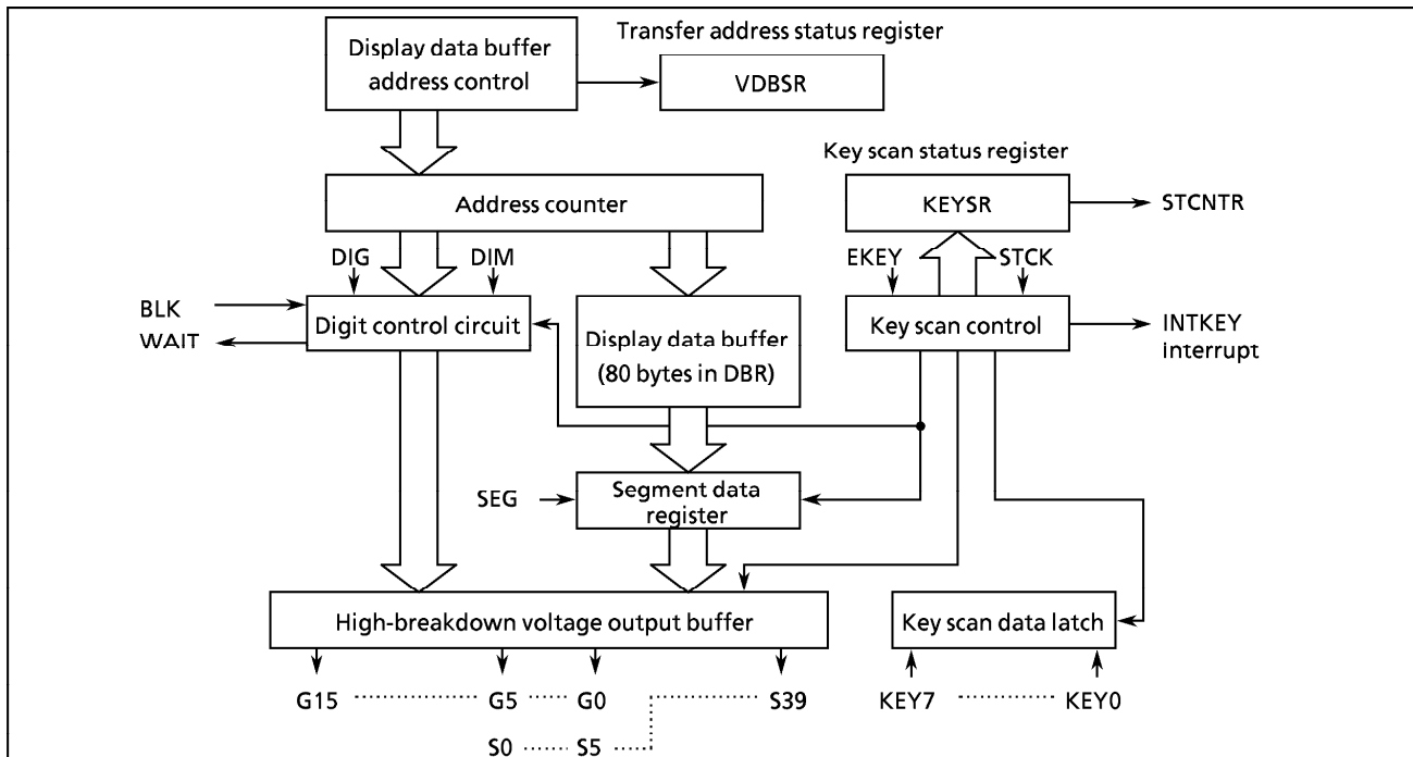
Figure 2-51. VFT
