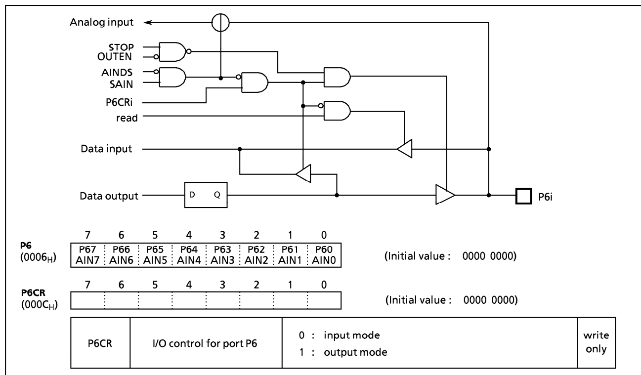
Figure 2-9. Port P6
