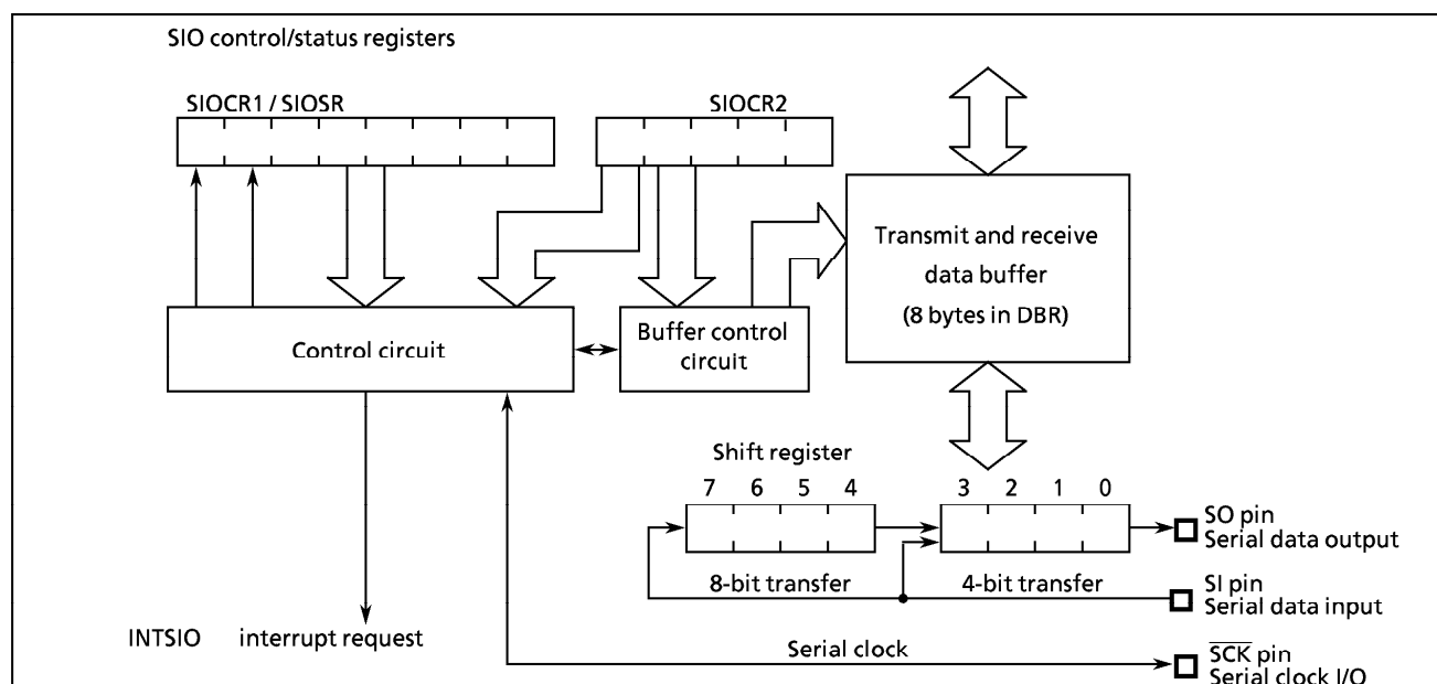
Figure 2-37. Serial Interfaces
