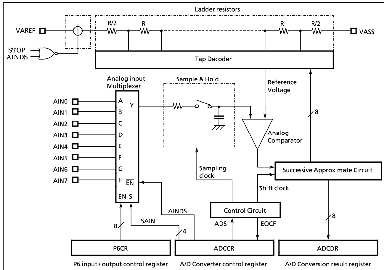
Figure 2-47. A/D Converter
