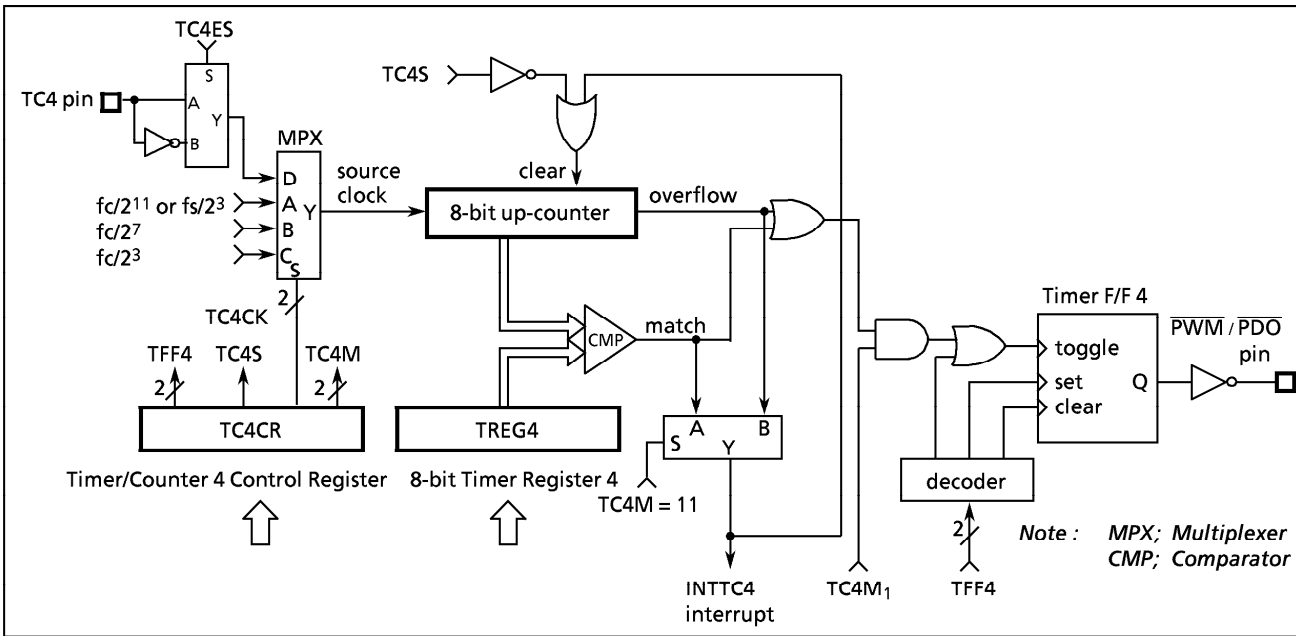
Figure 2-33. Timer/Counter 4
