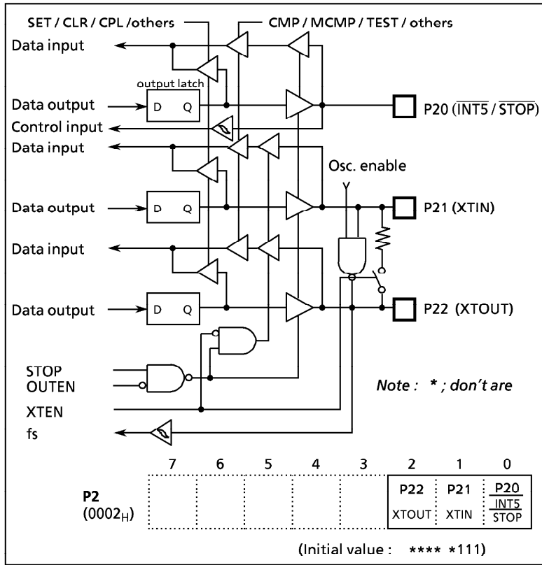
Figure 2-5. Port P2
