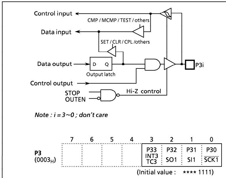
Figure 2-6. Port P3
