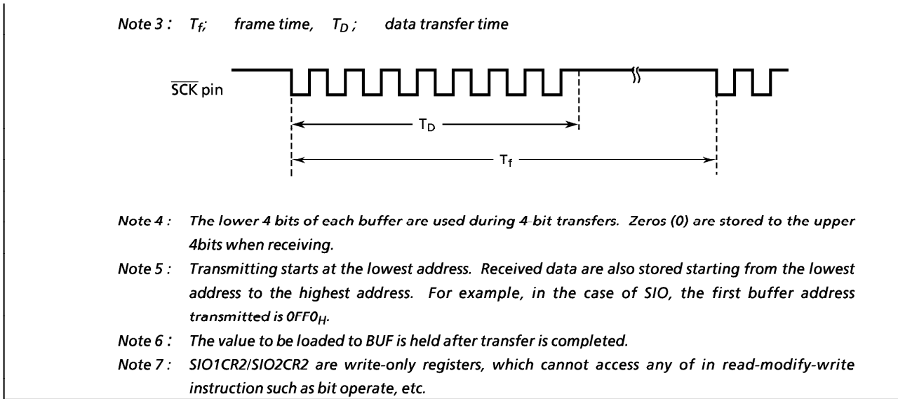
Figure 2-38. SIO Control Registers and Status Registers
