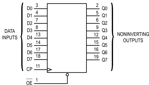
LOGIC DIAGRAM
