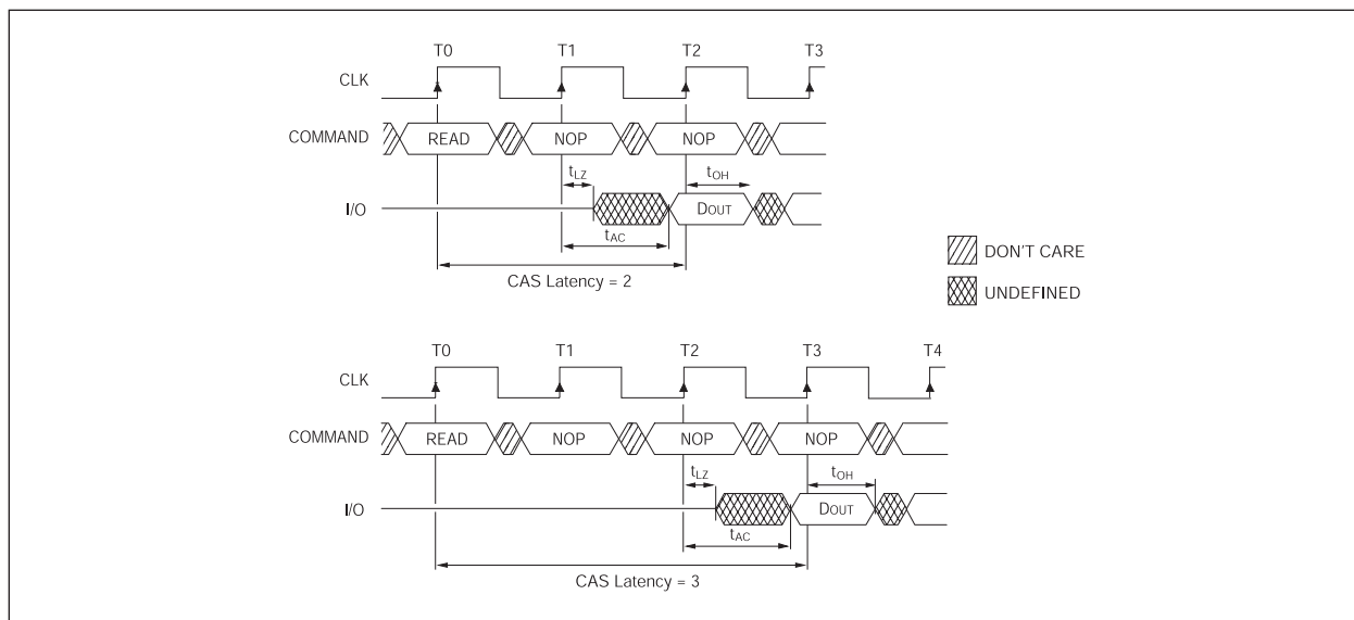
FIGURE 4 – CAS LATENCY
