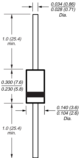
DO-204AC (DO-15)
