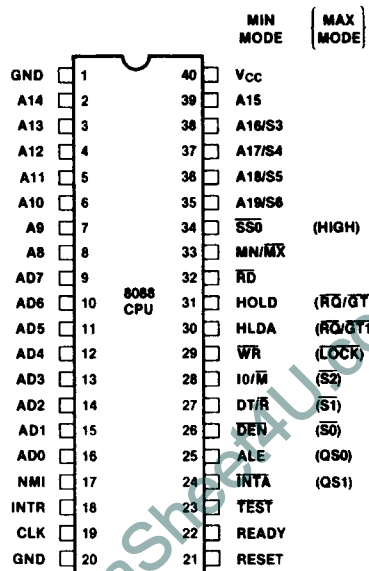
Figure 2. 8088 Pin Configuration
