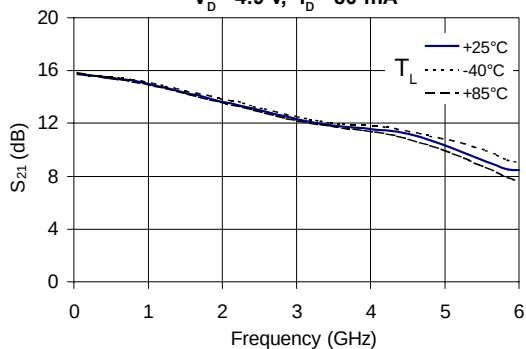
S_{21} vs. Frequency V_D = 4.9 v, I_D = 80 mA
