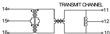
CIRCUIT 5
