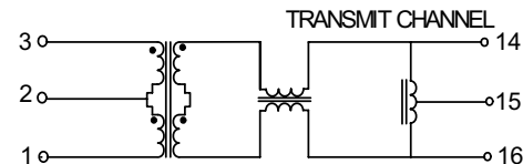
CIRCUIT 6
