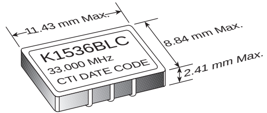
MECHANICAL DIMENSIONS
