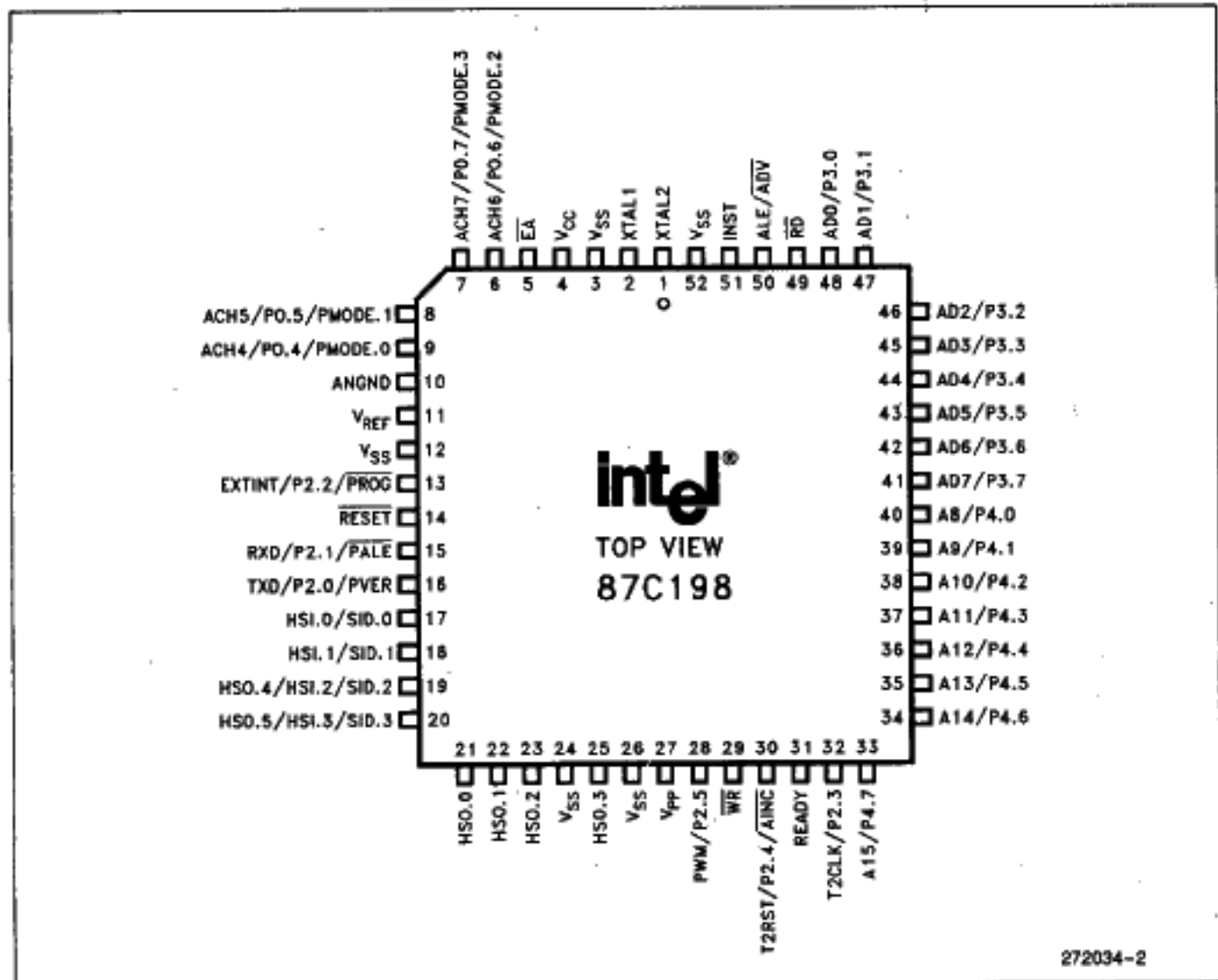
Figure 4. 52-Pin PLCC Package
