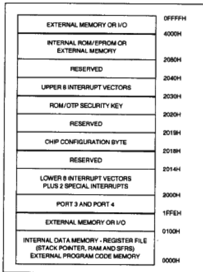
Figure 2. Memory Map
