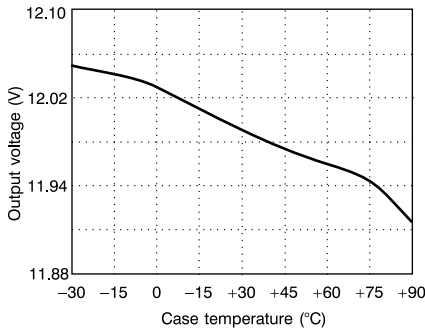
Temperature coefficient
