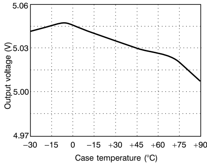
Temperature coefficient
