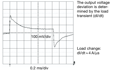
Dynamic load response (typ) @ +25^\circ\text{C}
