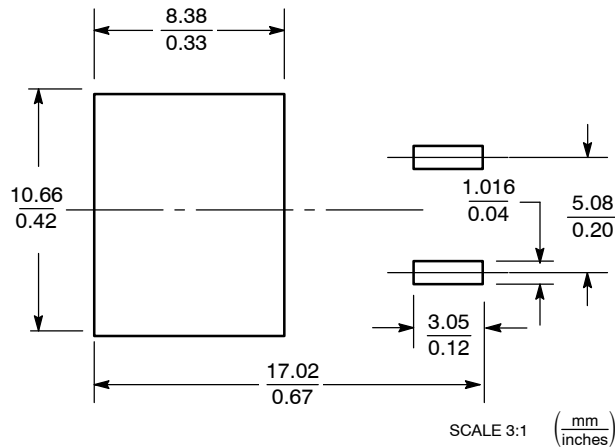
VIEW W-W 3
