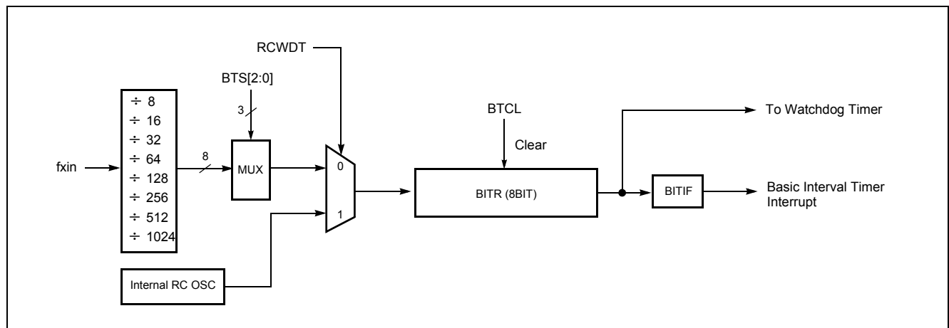
Figure 18-3 Block Diagram of Basic Interval Timer
