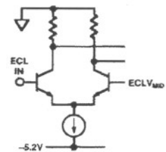
ECL Input Buffer
