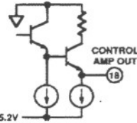
Control Amplifier Output
