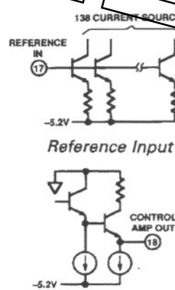
Control Amplifier Output
