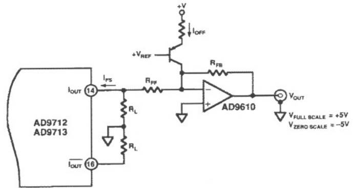
Figure 5. IV Conversion Using Current Feedback Amp
