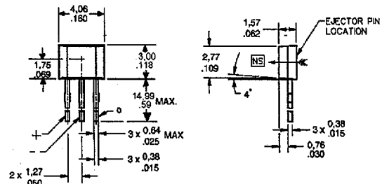
SURFACE MOUNT (-S) VERSION
