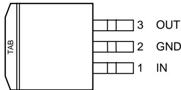
MIC5237-x.xBU (TO-263-3)
