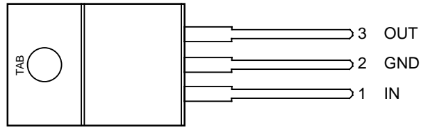
MIC5237-x.xBT (TO-220-3)
