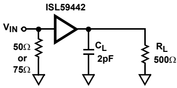
FIGURE 21A. TEST CIRCUIT WITH OPTIMAL OUTPUT LOAD
