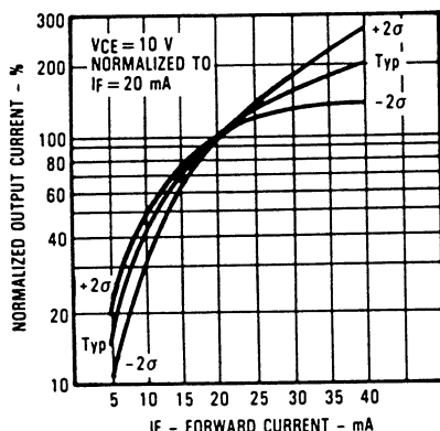
Normalized Output Current vs Forward Current
