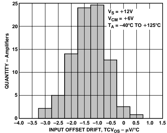
Figure 5. Input Offset Voltage Distribution ( TCV_{0s} )
