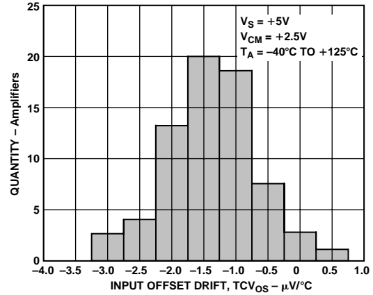
Figure 4. Input Offset Voltage Distribution ( TCV_{0s} )
