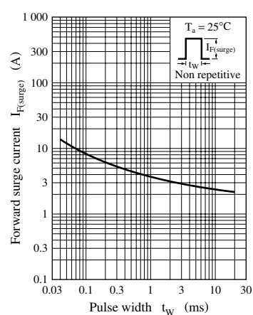
I_{F(\text{surge})} - t_w
