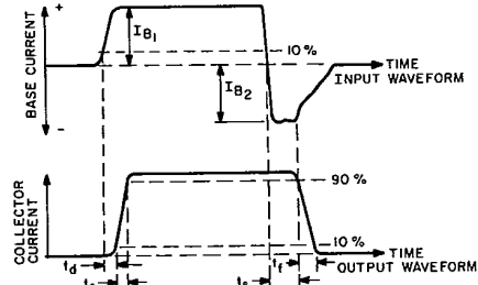
Fig. 18 - Oscilloscope display for measurement of switching times. (Circuit shown in Fig. 17).
