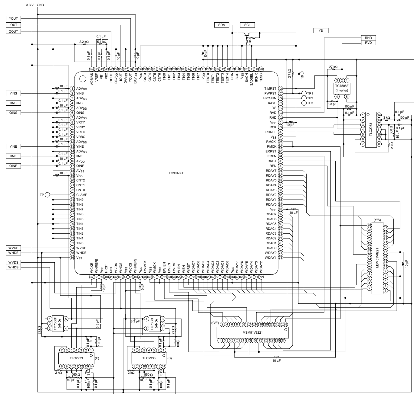
Application Circuit
