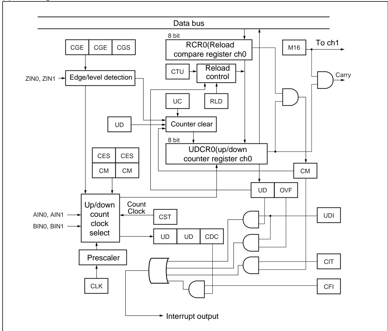
(3)Block diagram
