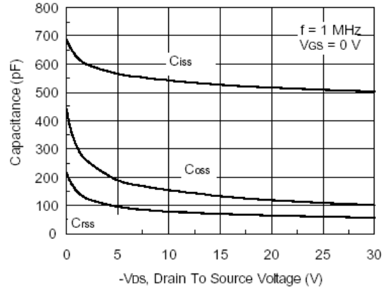
Figure 4. Capacitance Characteristics
