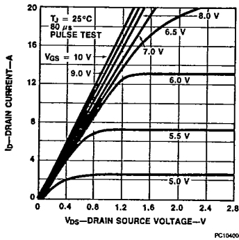
Figure 1 Output Characteristics
