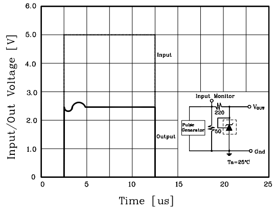
Fig. 9 Pulse reponse
