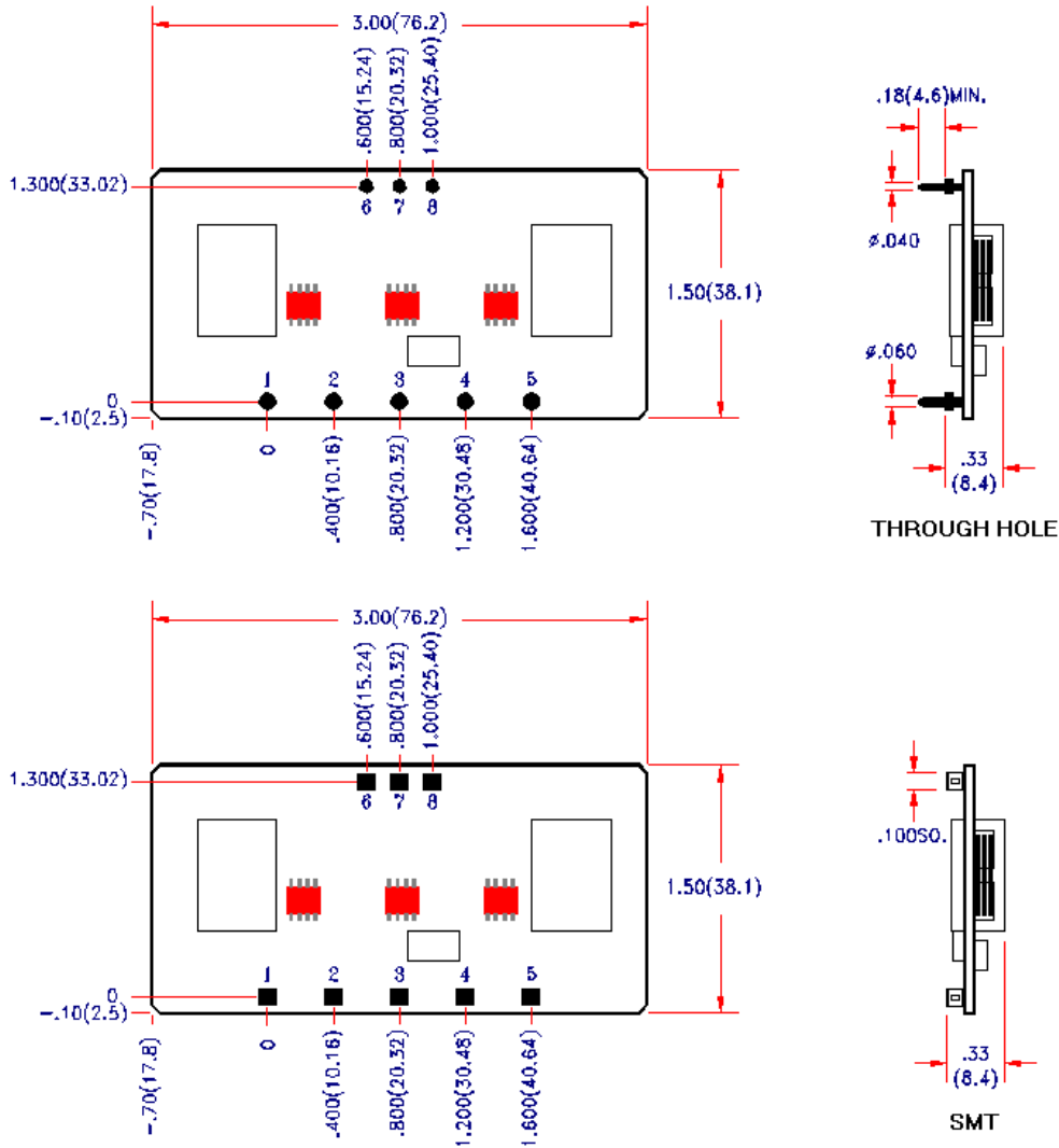
PIN VIEW
