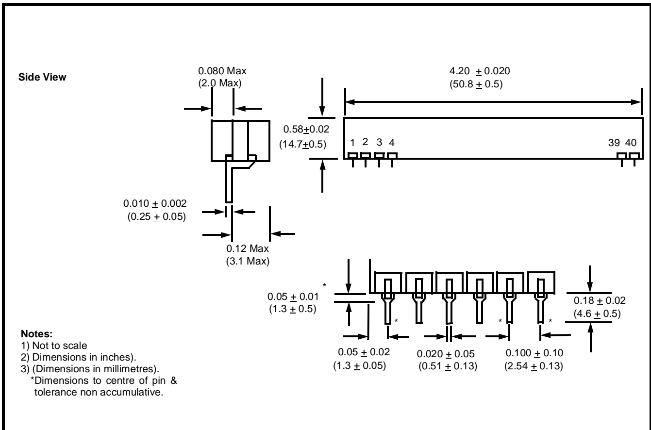
Figure 8 - Mechanical Data
