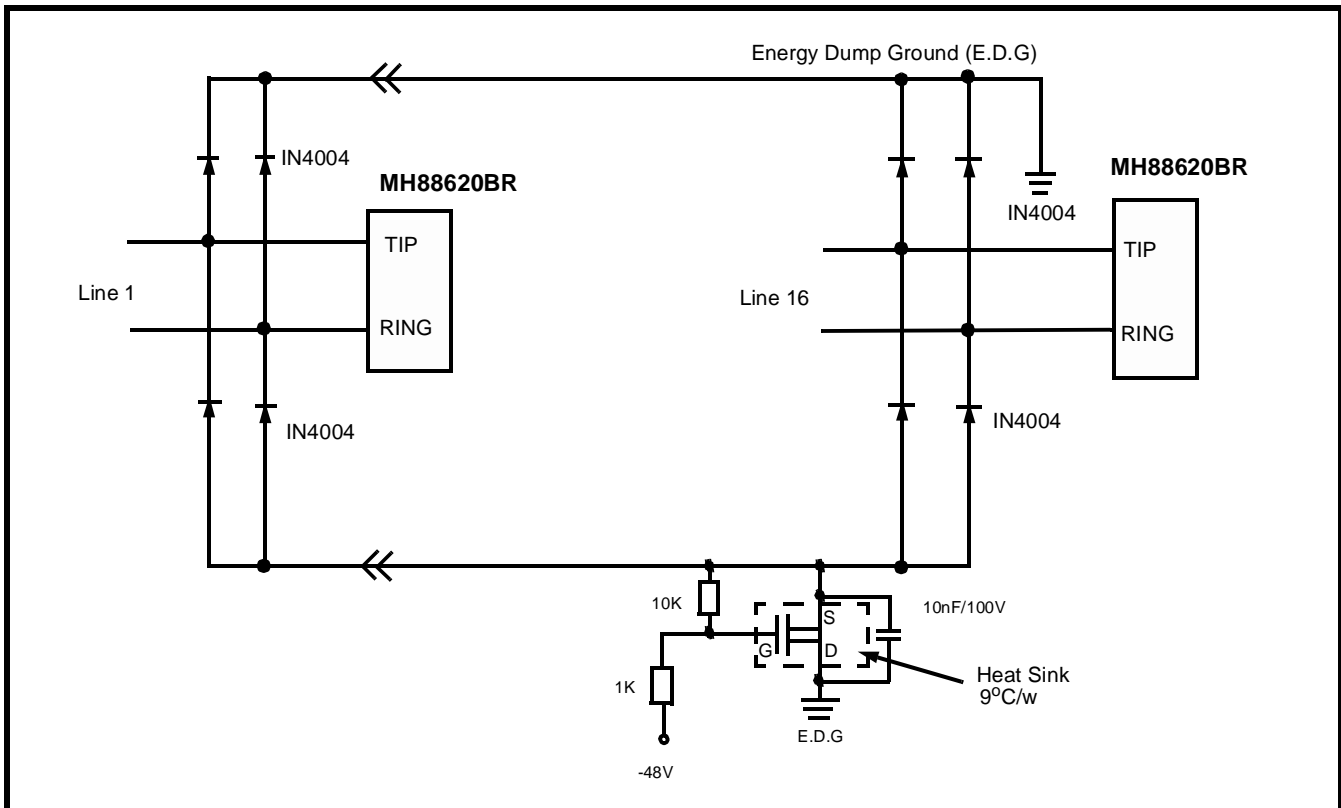
Figure 7c -16 Lines Circuit Configuration
