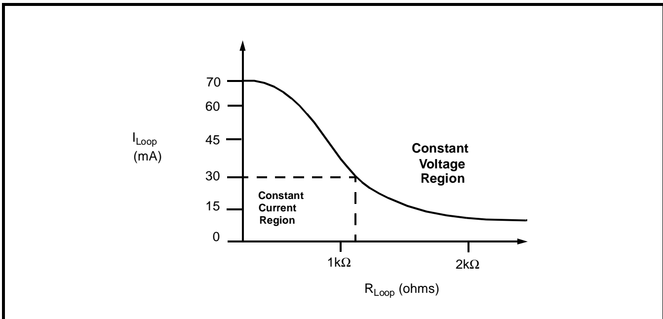
Graph 1 - I_{Loop}/R_{Loop} Characteristics
