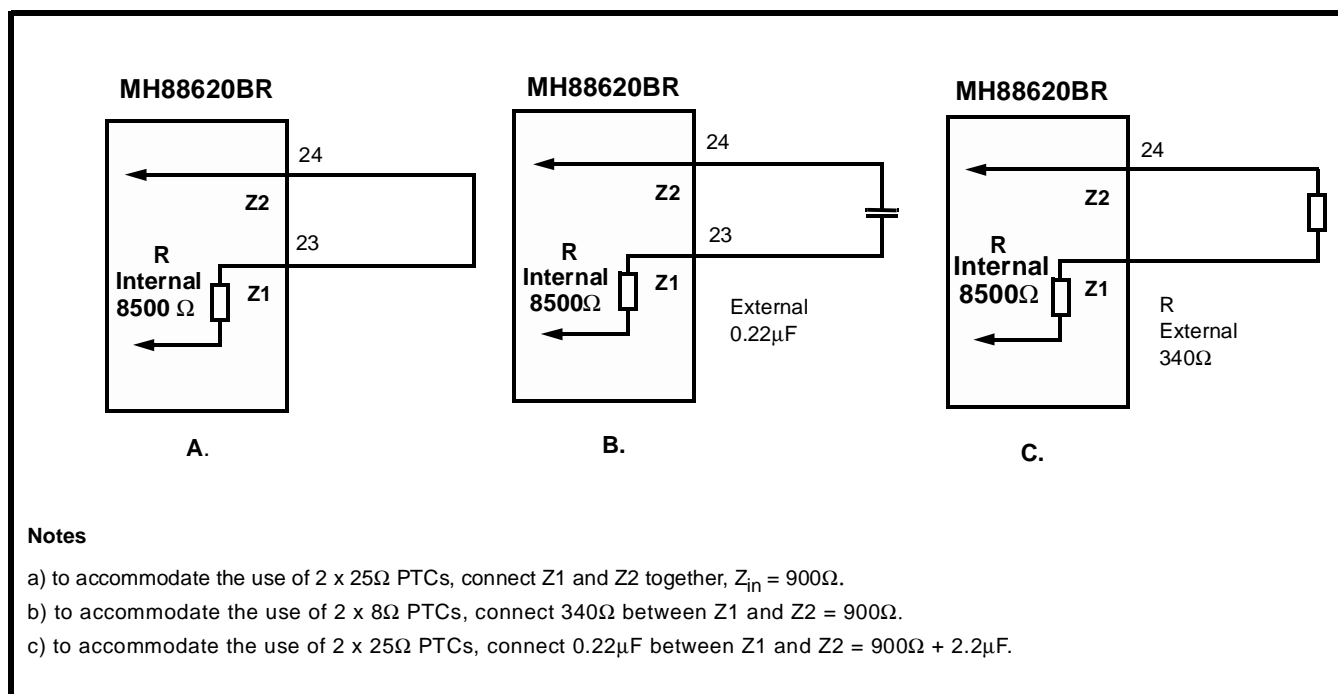
Figure 3 - Input Impedance ( Z_{in} ) setting
