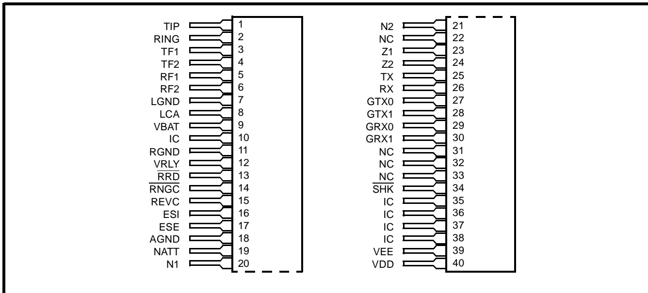
Figure 2 - Pin Connections
