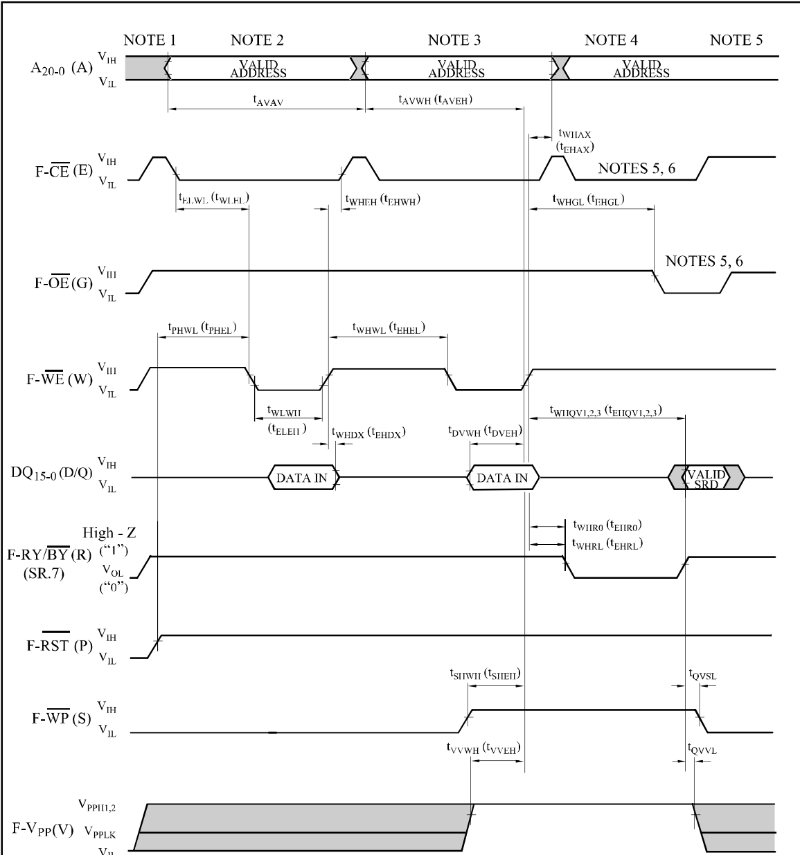
AC Waveform for Write Operations(F-WE / F-CE Controlled)
