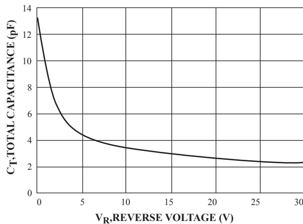
FIG.4 Total Capacitance
