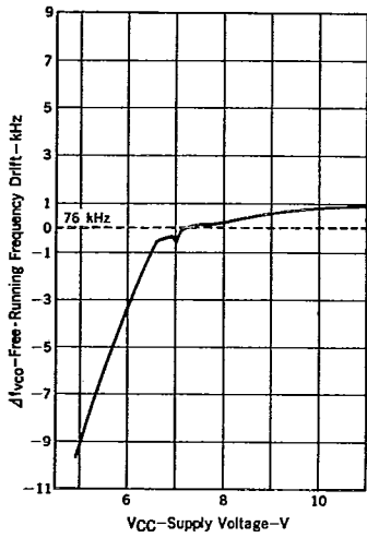
FREE RUNNING FREQUENCY vs. SUPPLY VOLTAGE
