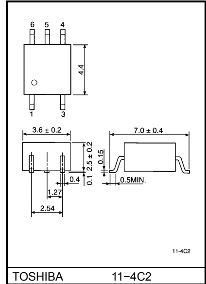
TOSHIBA 11-4C2 Weight: 0.09g
