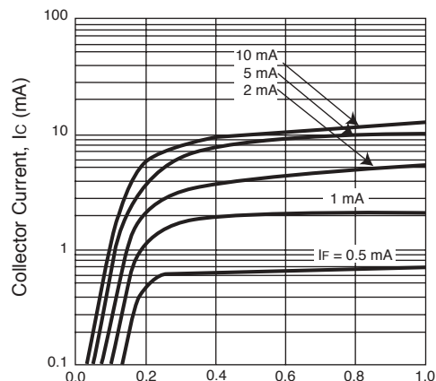
Collector Saturation Voltage, V_{CE(sat)} (V)
