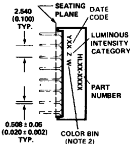
SIDE VIEW E, F, G, H
