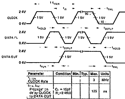
Figure 1. Switching Characteristics HDSP-2490/-2491/-2492/-2493 (T A = -20°C to -85°C)
