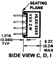
SIDE VIEW C, D, I
