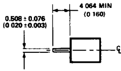
END VIEW A, B
