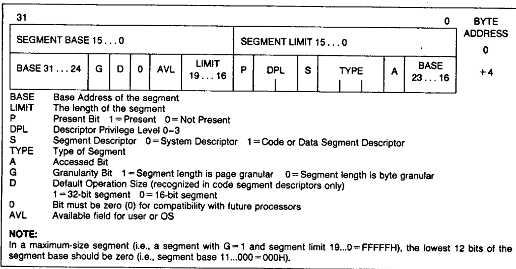
Figure 4.5. Segment Descriptors
