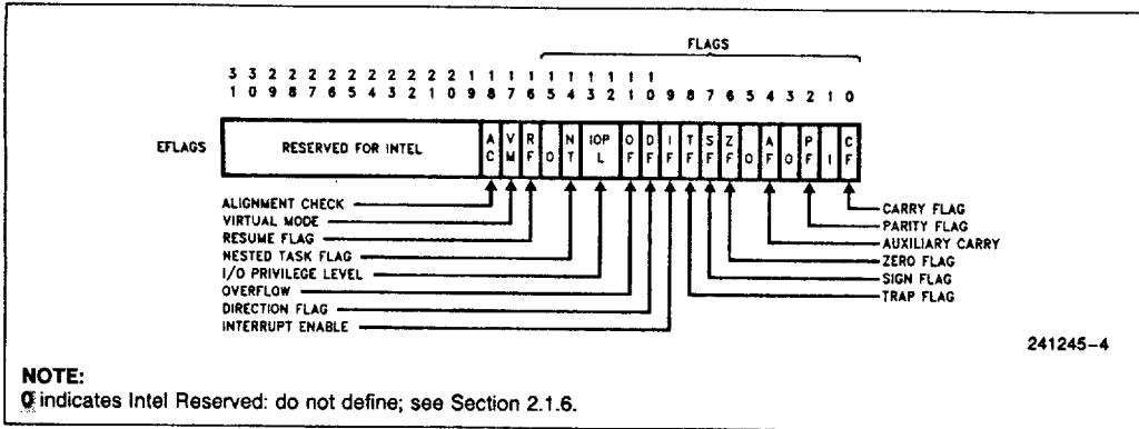
Figure 2.2. Flags Register
