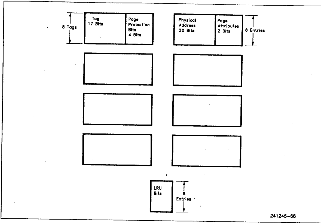
Figure 8.3. TLB Organization
