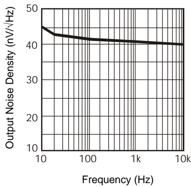
OUTPUT NOISE-VOLTAGE DENSITY vs. FREQUENCY
