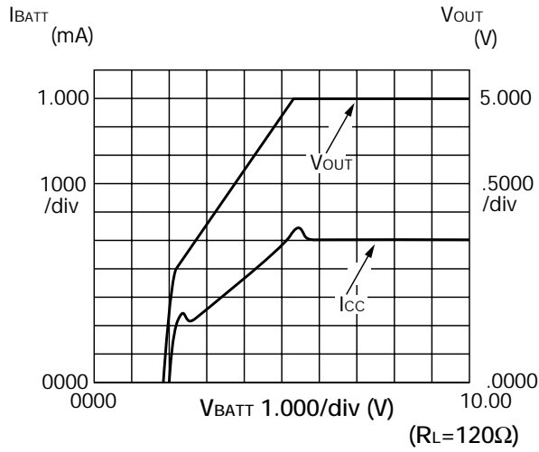
■ Output voltage and current consumption for V_{CC} voltage supply
