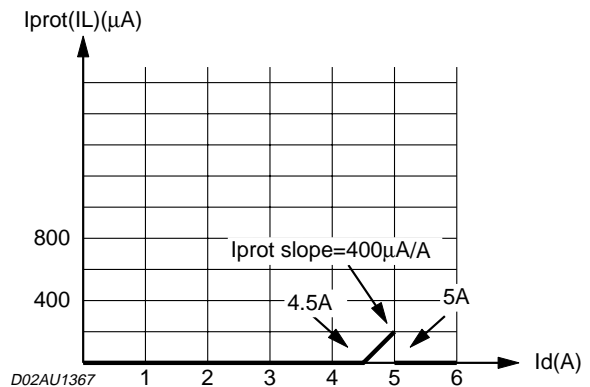
Figure 4. Protection current behaviour I_{prot}(I_L)
