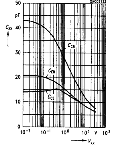
Figure 11. Transistor capacitance (typ.) T_A=25^\circ\text{C} , f=1 MHz, C_{CE}=f(V_{CE}) C_{CB}=f(V_{CB}) , C_{EB}=f(V_{EB})
