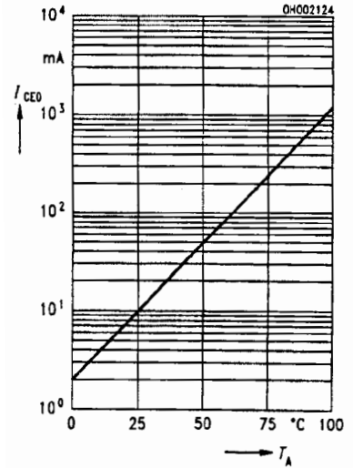
Figure 12. Collector-emitter leakage current I_F=0 , V_{CE}=10 V, I_{CEO}=f(T_A)
