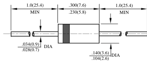
DO-15
