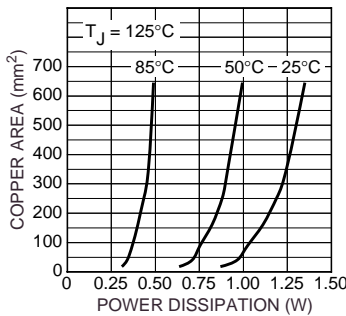
Figure 9. Copper Area vs. Power-SOIC Power Dissipation ( T_A )
