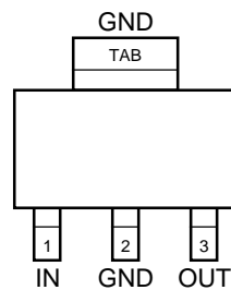
SOT-223 (S)
