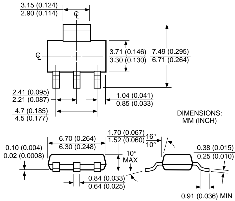
SOT-223 (S)
