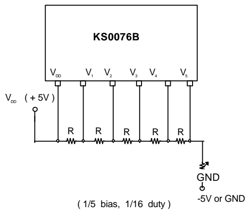
BIAS VOLTAGE
