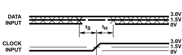
FIGURE 9. SETUP AND HOLD TIME
